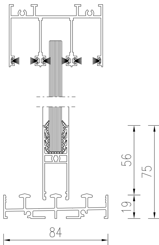
ALUPROF MB-OpenSlide
